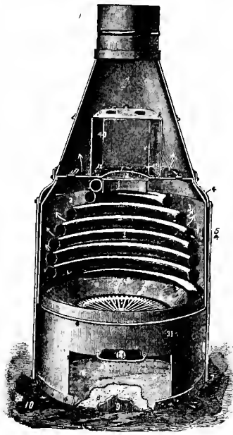
Fig. 2866. Sectional View. THE "FIRE-PROOF" HEATER.
